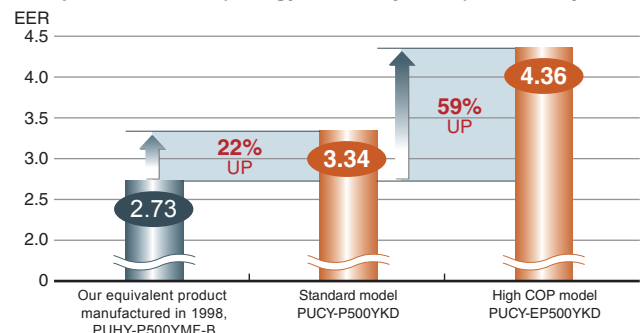
Comparison of EER (Energy Efficiency Ratio) – 20 HP system
