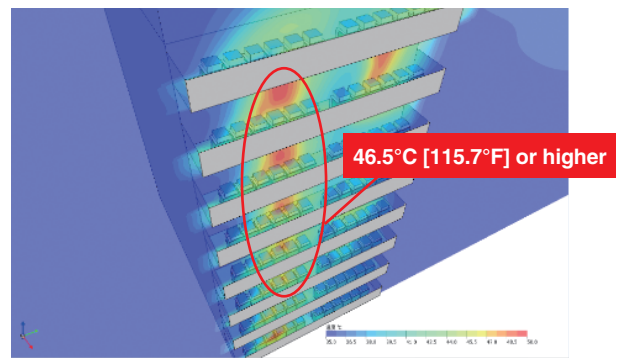
Installation on each floor a high-rise building
