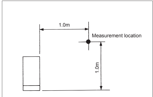
■ PFFY-P-YM(H)-E, PFFY-P-YM-E-F
