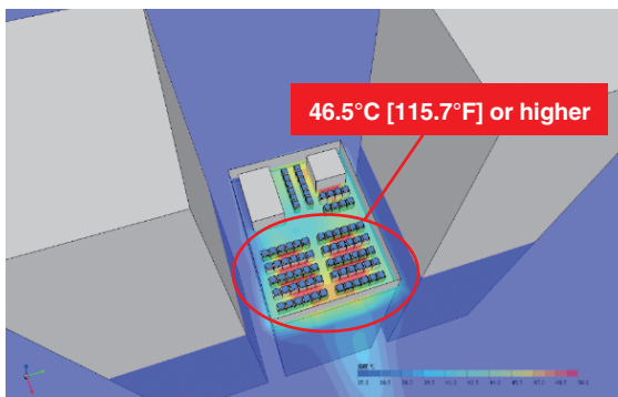
Built-up area with buildings and outdoor units
