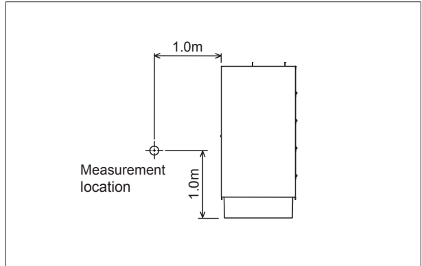
■ PFFY-P-YM(H)-E, PFFY-P-YM-E-F
